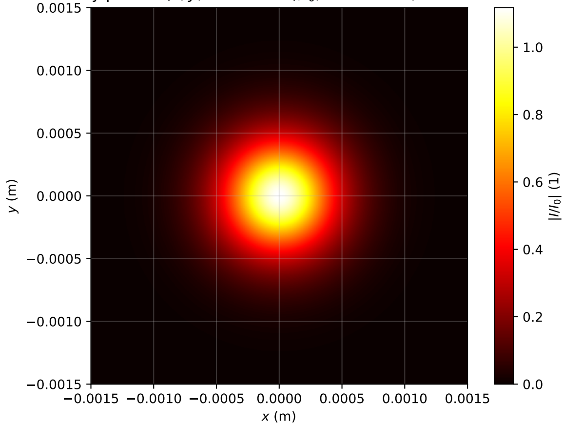
Intensity profile I(x, y, z = 0.876m)/I_0 , P_{in}=0.6P_{cr} , artificial time
